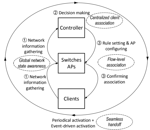
Fig. 3: Workflow of centralized client association in SDWLAN.
