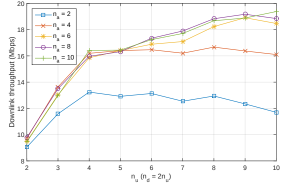
Fig. 6: Downlink throughput with different n_a .
