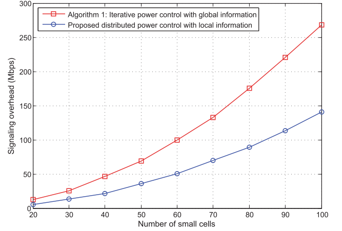
Fig. 7. Signaling overhead analysis.
