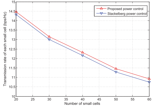
Fig. 5. The performance evaluation of average transmission rate for different solutions versus the number of small cells.
