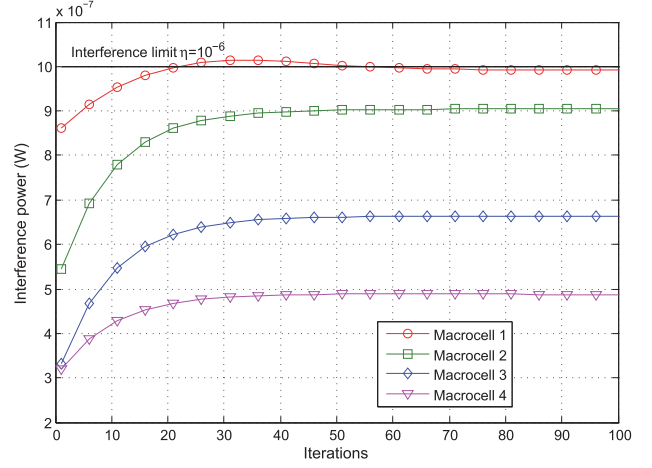
Fig. 4. The evolution of received interference by macrocells when the number of small cells is 50.
