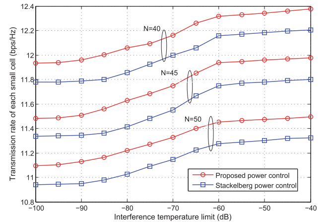
Fig. 9. The performance evaluation of average transmission rate for different solutions versus the interference temperature limit.
