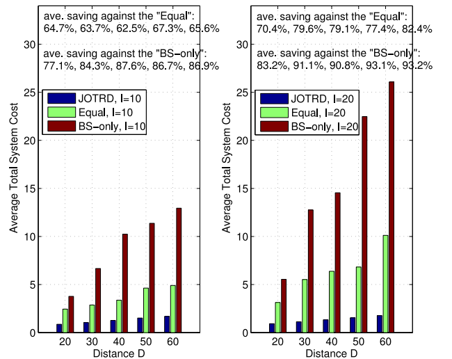
Fig. 7. Advantage of the MDs' cooperations in saving the total system cost. We plot the average total system versus different distance D = 20, 30, \dots, 60 . Left subplot: We fix the number of MDs I = 10 . Right subplot: I = 20 . For each tested case, the result (i.e., the total system cost) is averaged over 200 randomly generated network scenarios. Besides, the numbers illustrated on the top of each subplot denote the average saving ratios of the total system cost by using Algorithm JOTRD against the equal-distribution approach and the BS-only approach, respectively.
