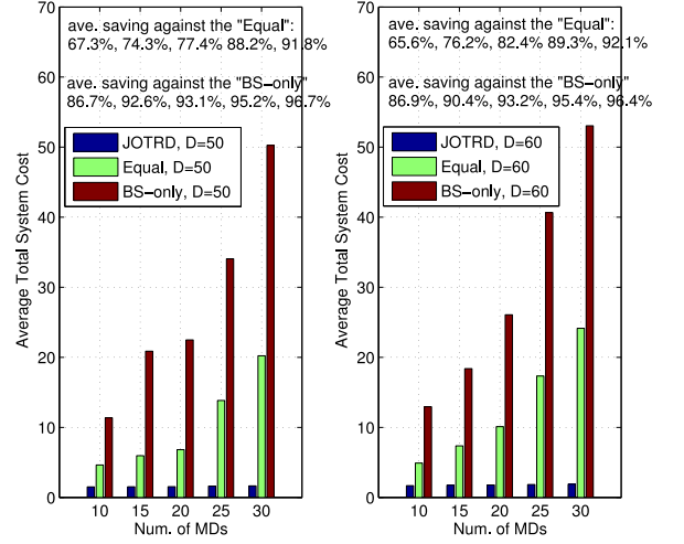
Fig. 6. Advantage of saving the total system cost by using the optimal MDs cooperations. We plot the average total system versus different number of the MDs I = 10, 15, \dots, 30 . Left subplot: the distance between the BS and the central of the circle D = 50 . Right subplot: D = 60 . For each tested case, the result (i.e., the total system cost) is averaged over 200 randomly generated network scenarios. The numbers illustrated on the top of each subplot denote the average saving ratios of the total system cost by using Algorithm JOTRD against the Equal-distribution approach and the BS-only approach, respectively.
