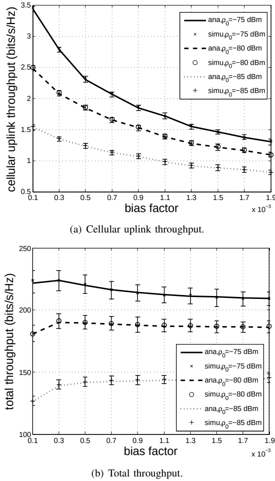
Figure 6. Throughput performance w.r.t. \varphi .
