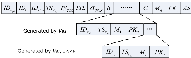
Fig. 4. The format of the V_{p1} .
