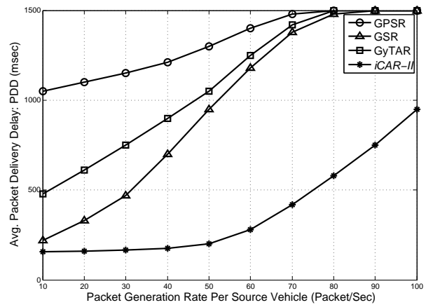
Fig. 13. Average Packet Delivery Delay ( PDD ) using 4 RSUs and vehicle density of 70 vehicle/lane.km
