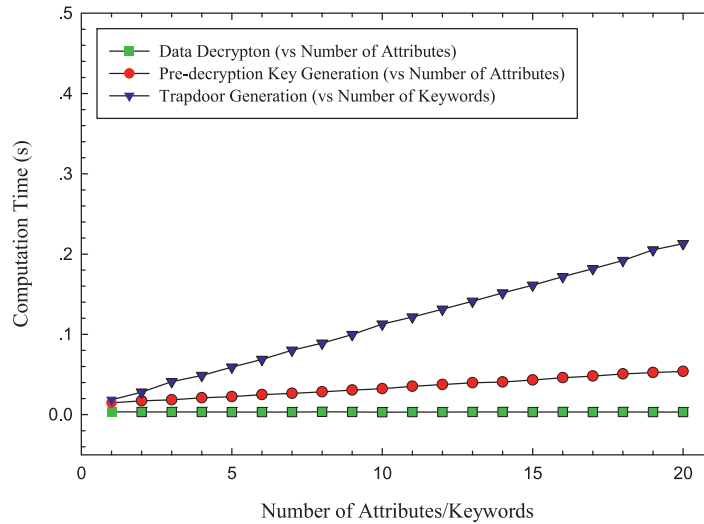
Fig. 4. Computation overhead on the subscribers.
