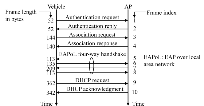
FIGURE 1. Management frames exchanged between a vehicle and an AP based on the WPA2-PSK mode for authentication ( N_f = 10 ).
