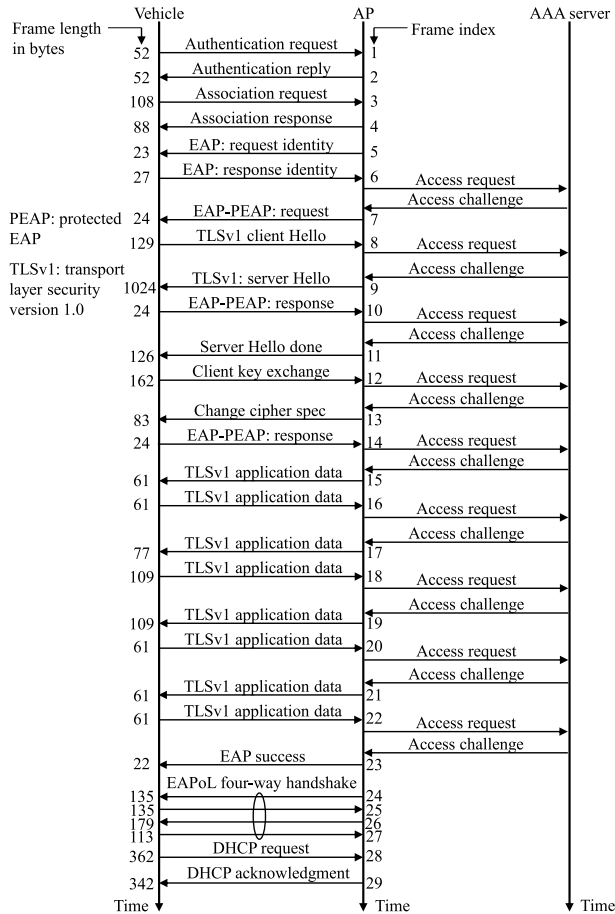
FIGURE 2. Management frames exchanged between a vehicle and an AP based on the WPA2-802.1X mode for authentication ( N_f = 29 ).
