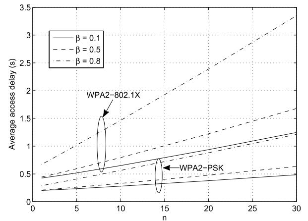
FIGURE 5. Comparison of the access delay performance for the WPA2-802.1X and WPA2-PSK authentication mechanisms.
