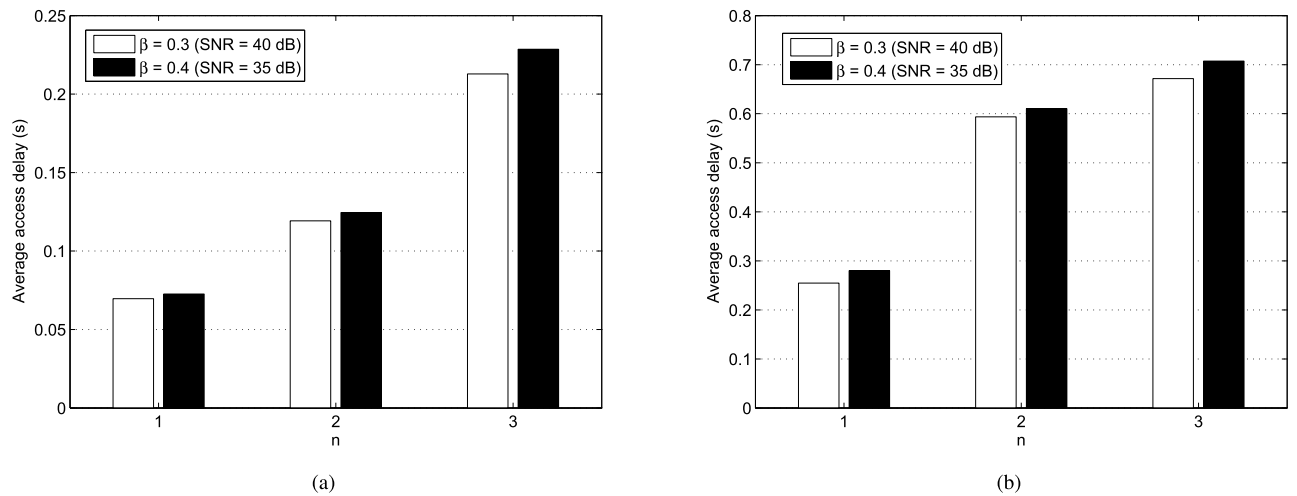
FIGURE 8. Experimental results of the access delay when the WPA-PSK mode and the WPA2-802.1X standard are employed for authentication. (a) WPA2-PSK. (b) WPA2-802.1X.
