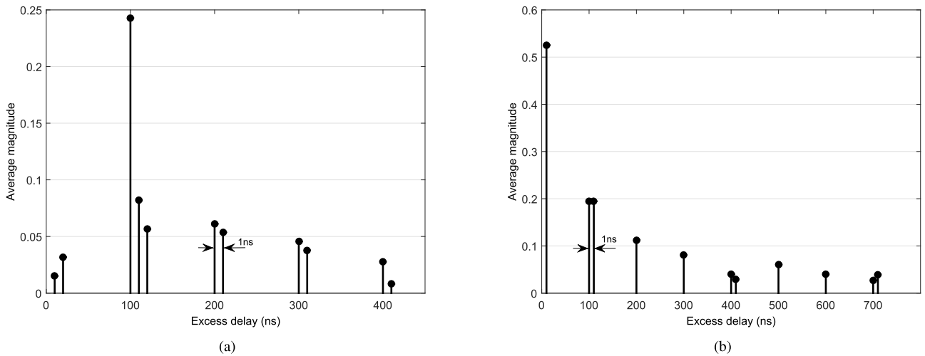
FIGURE 7. The V2R and V2V channel models used in the experiments. The average magnitude of the LoS tap is normalized to unity (the LoS tap is not shown). (a) V2R channel model. (b) V2V channel model.
