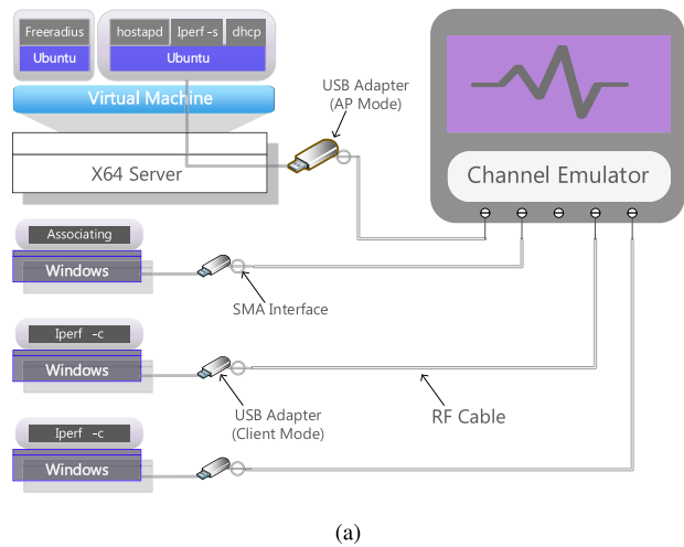
FIGURE 6. Experiment framework. (a) Schematic diagram. (b) Testbed.
