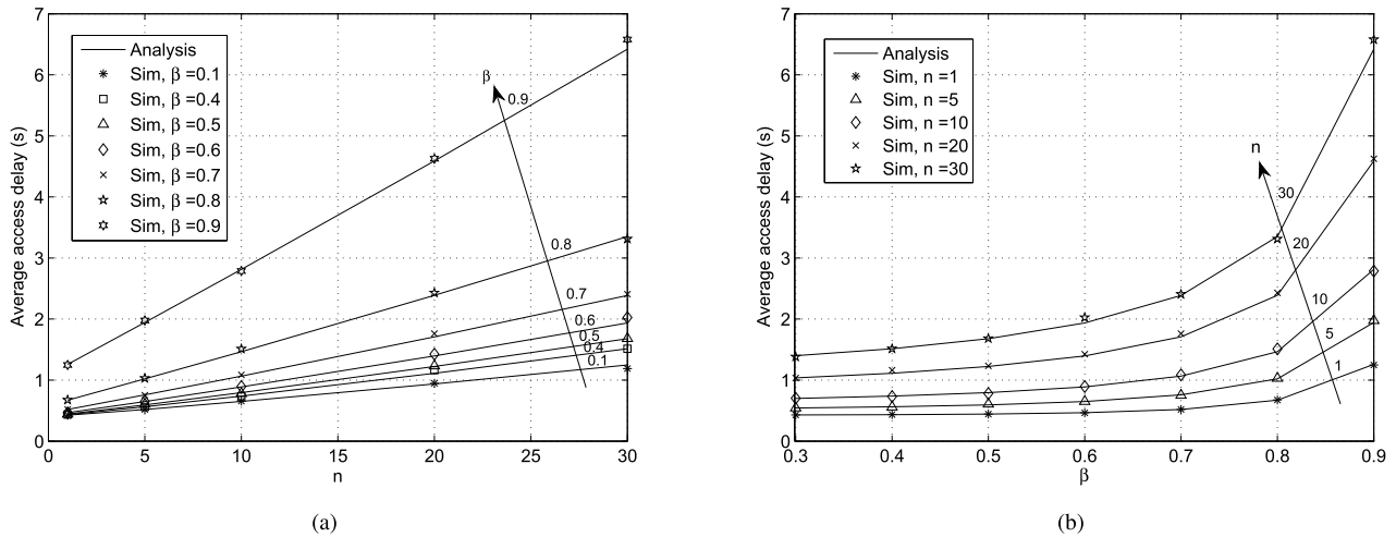
FIGURE 4. Analytical and simulations (Sim) results of the access delay when the WPA2-802.1X standard is employed for authentication. (a) Average access delay versus n . (b) Average access delay versus \beta .
