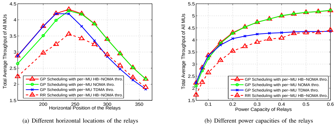
Fig. 12: Performance advantage of the GP-based scheduling with the HB-NOMA relay. Each point denotes the result after 400 time-slots.
