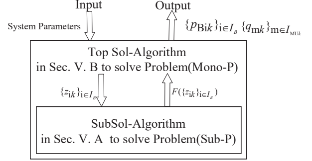
Fig. 4: Connection between TopSol-Algorithm and SubSol-Algorithm
