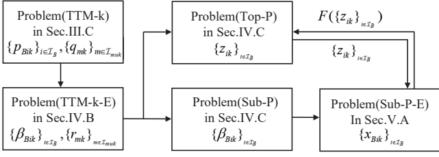
Fig. 3: Decomposition of Problem (TTM-k) into Problem (Top-P) and Problem (Sub-P).
