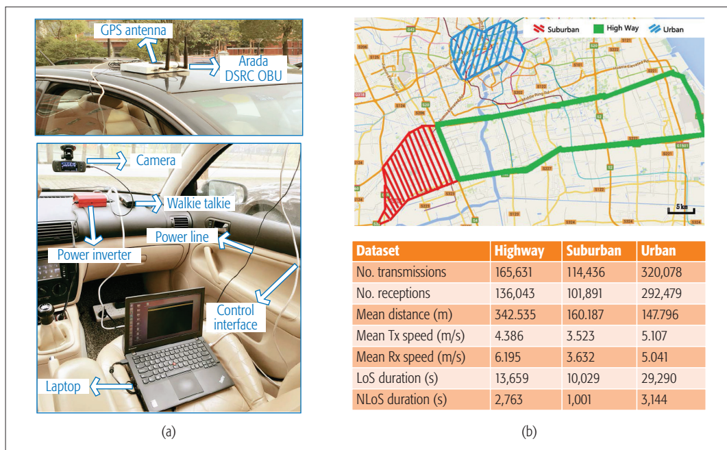
FIGURE 1. Illustration of data collection: a) experimental devices; b) data collection environments and dataset details.
