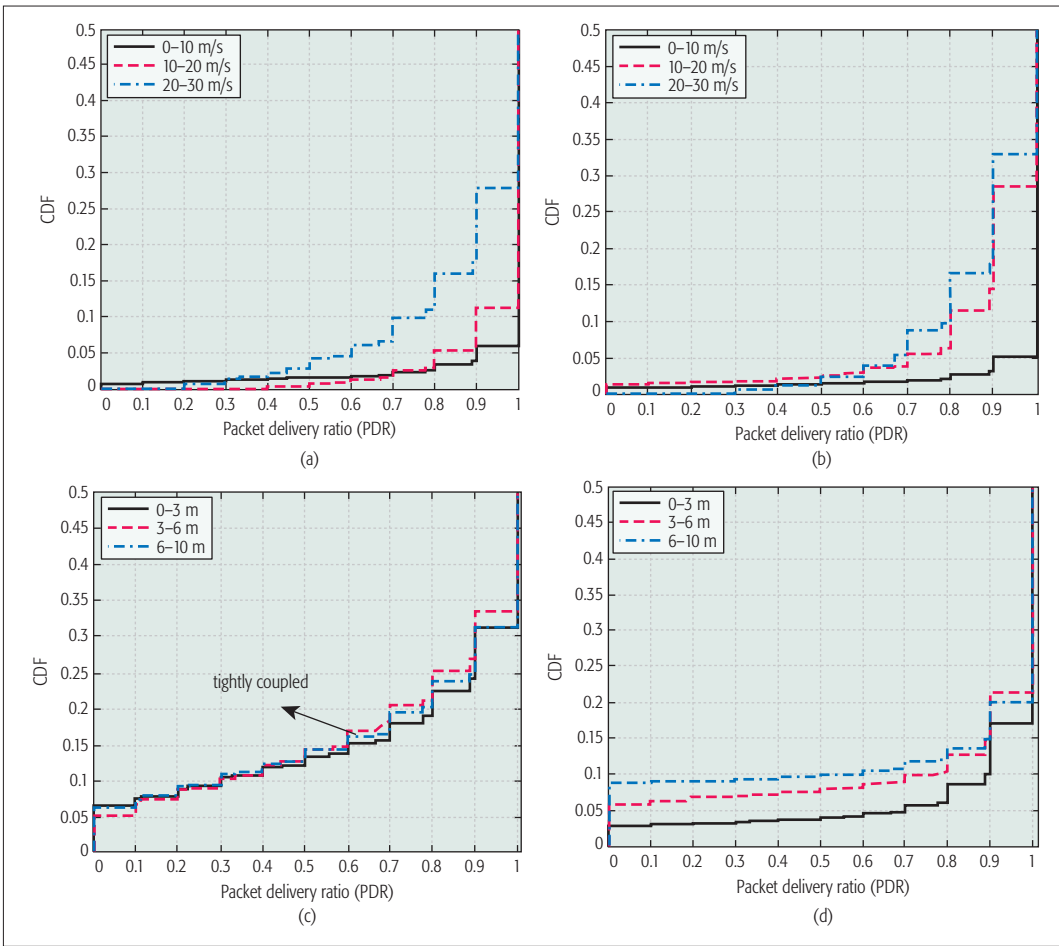
FIGURE 3. CDFs of PDR at different effect velocity and relative altitude ranges: a) highway: at different effect velocity ranges; b) urban: at different effect velocity ranges; c) highway: at different relative altitude ranges; d) urban: at different relative altitude ranges
