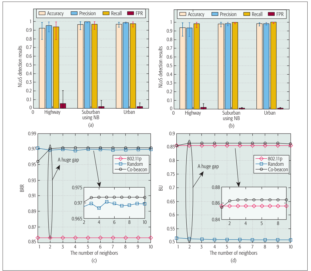
FIGURE 6. Simulation results: a) NLoS detection results with NB; b) NLoS detection results with SVM; c) BRR vs. the number of neighbors; d) BU vs. the number of neighbors.
