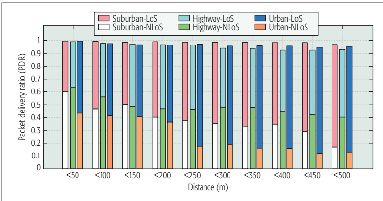
FIGURE 4. Average PDR vs. distance under LoS/NLoS conditions.
