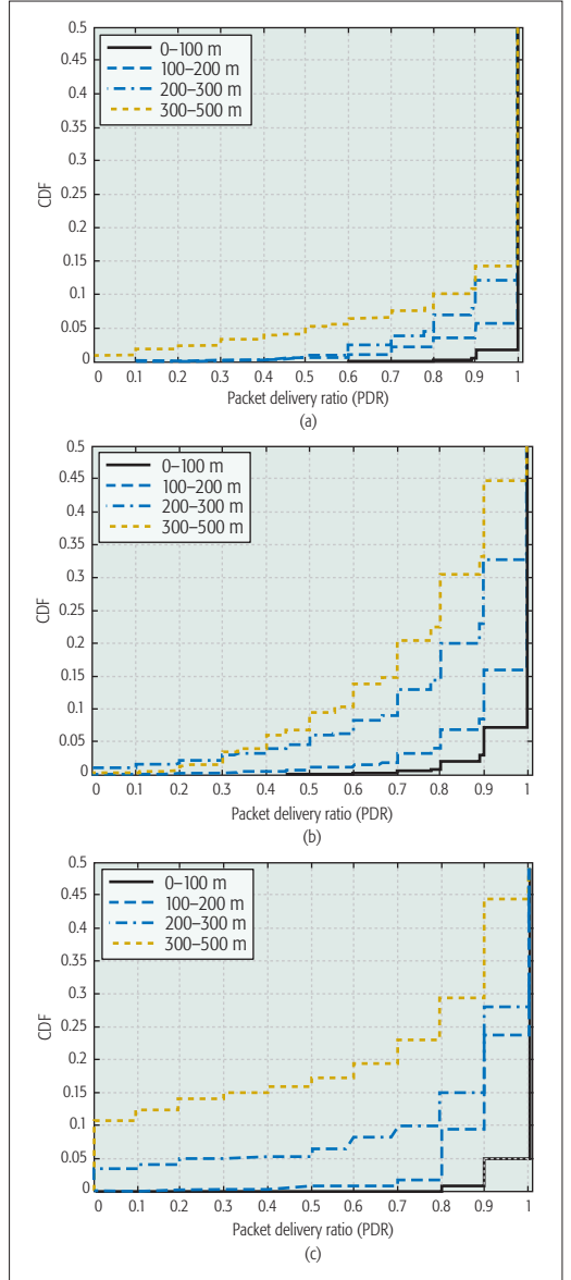
FIGURE 2. CDFs of PDR within different separation distance ranges: a) suburban; b) highway; c) urban.
