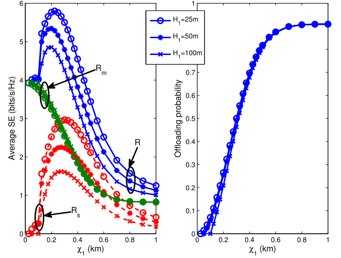
Fig. 3. Average SE and offloading probability w.r.t \chi_1 .
