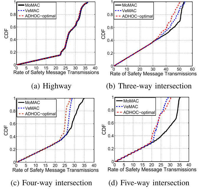
Fig. 13. CDFs of rate of safety message transmissions in different scenarios under moderate traffic condition.
