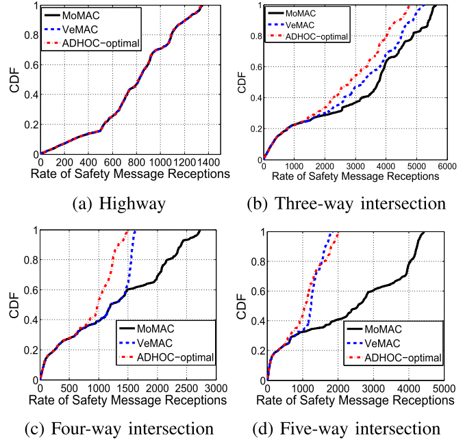
Fig. 14. CDFs of rate of safety message receptions in different scenarios under moderate traffic condition.
