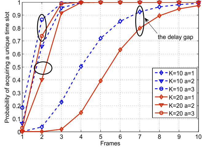
Fig. 10. The access delay under unstable state.
