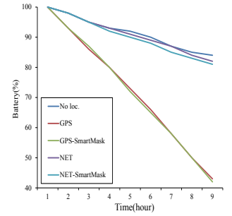
Fig. 10: Energy overhead
