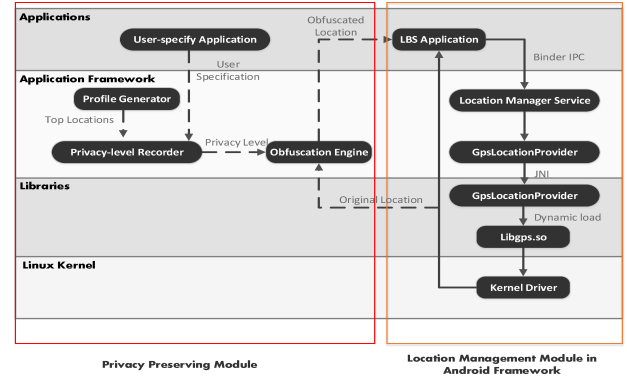
Fig. 6: SmartMask architecture
