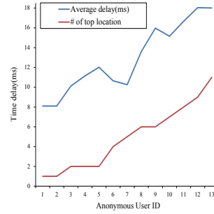
Fig. 9: Time delay
