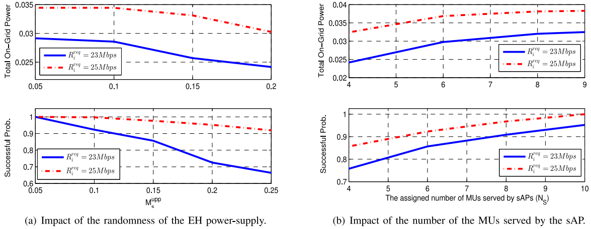
Fig. 7. Optimal solution of Problem (OGPM) under different parameter-settings.
