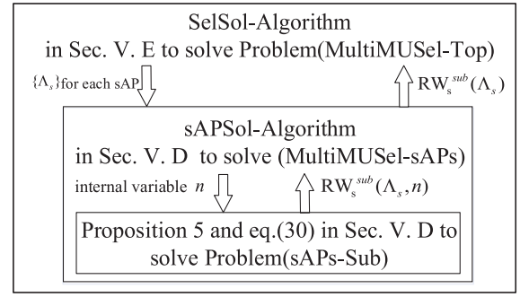
Fig. 4. Connections between SelSol-Algorithm, sAPSol-Algorithm, and Proposition 5 and eq. (31).
