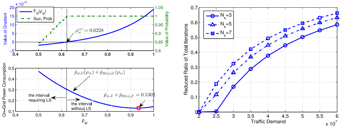
(a) An illustrative example of executing ADLS-Algorithm. Top: Example of F(r_{si}) . Bottom: Total on-grid power. (b) Advantage of reducing the number of iterations used by ADLS-Algorithm in comparison with using LS-Algorithm.
