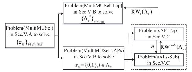
Fig. 3. Decomposition of Problem (MultiMUSel) into Problem (MultiMUSel-Top) on the top and Problem (MultiMUSel-sAPs) for each sAP s at the bottom. Problem (MultiMUSel-sAPs) is further decomposed into Problem (sAP-Top) and Problem (sAP-Sub) in Section V-C.
