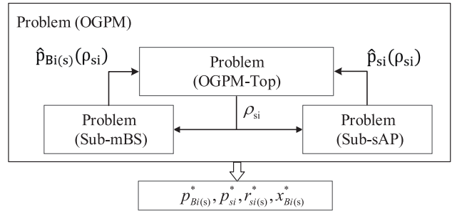
Fig. 2. Decomposition of Problem (OGPM) into a top-problem (i.e., Problem (OGPM-Top)) and two subproblems (i.e., Problem (Sub-mBS) and Problem (Sub-sAP)).
