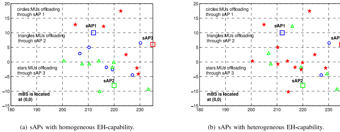
Fig. 8. Examples of the optimal MU-selection solution of Problem (MultiMUSel) under \mu = 0.025\$/Mbps and \pi = 0.002\$/KW .
