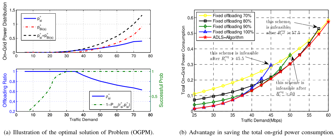
Fig. 6. Illustration of the optimal offloading solution and the advantage in reducing the total on-grid power consumption.
