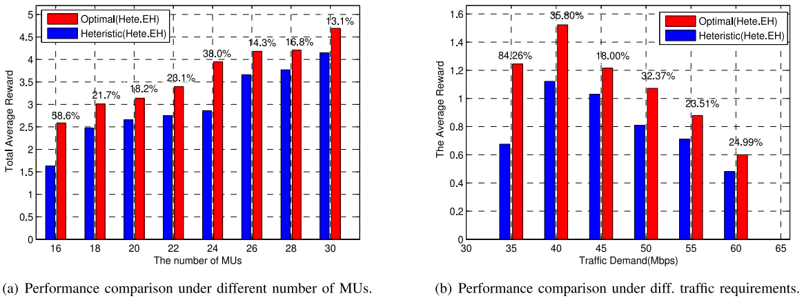
Fig. 9. Performance advantage of the optimal MU-selection solution.
