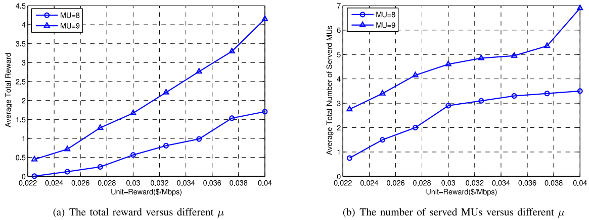
Fig. 10. Optimal MU-selection solution under different Marginal Reward.
