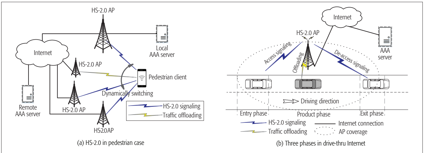
FIGURE 2. HS-2.0 enabled traffic offloading cases.
