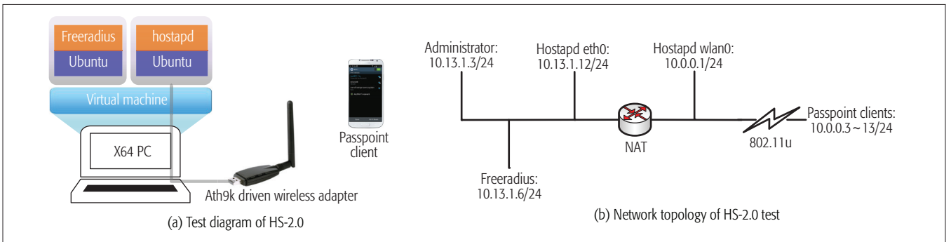
FIGURE 3. HS-2.0 test diagram and network topology.
