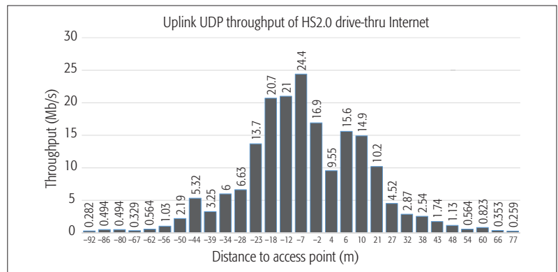
FIGURE 4. HS-2.0 drive-thru Internet measurement results.
