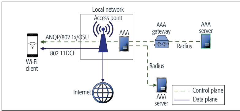
FIGURE 1. System architecture of HS-2.0 for WiFi networks.
