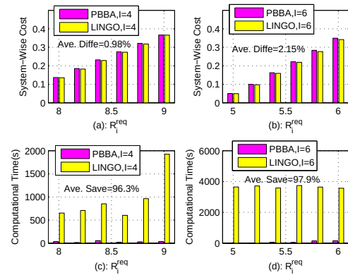
Fig. 4: Performance of PBBA-Algorithm to solve top-problem (BA) for the cases of I = 4 and I = 6 .
