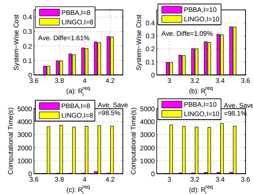
Fig. 5: Performance of PBBA-Algorithm to solve top-problem (BA) for the cases of I = 8 and I = 10 .
