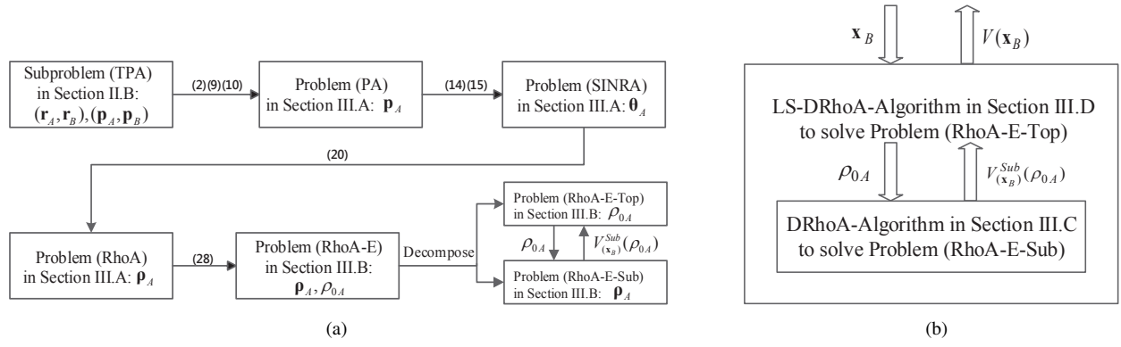
Fig. 2: Subfigure (a): A series of equivalent transformations that transform subproblem (TPA) to Problems (RhoA-E-Top) and (RhoA-E-Sub). Subfigure (b): Connections between our proposed LS-DRhoA-Algorithm and its subroutine DRhoA-Algorithm.
