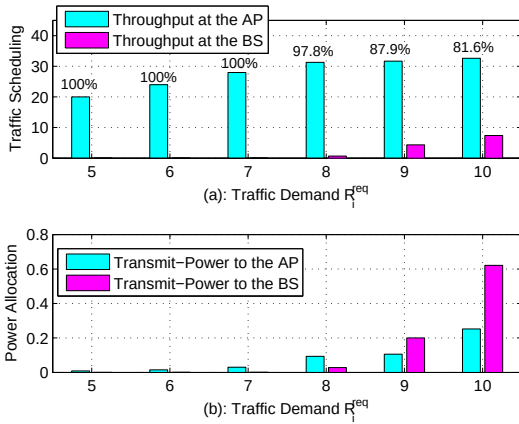
Fig. 6: Optimal offloading solution (MUs' traffic scheduling & power allocation) for the 4-MU scenario. (a): the MUs' throughput to the AP and BS; (b): the MUs' total transmit-power consumptions to the AP and BS.
