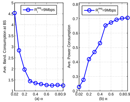
Fig. 10: Performance under different \alpha . We set I = 4 , and each value in this figure denotes the average result of 100 random sets of the MUs' locations and channel power gains. (a): Average bandwidth usage at the BS; (b): Average total power consumption of all MUs.
