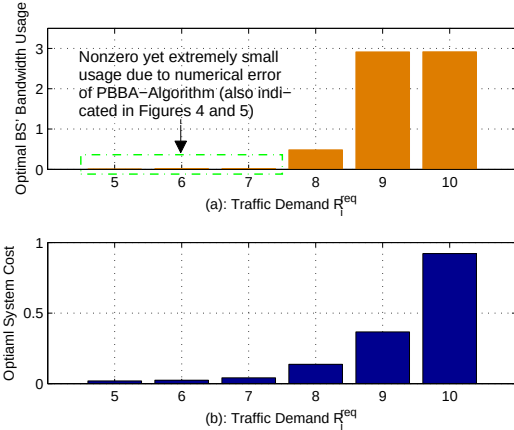
Fig. 7: Optimal offloading solution (the BS' bandwidth usage and overall system cost) for the 4-MU scenario. Subplot (a): the BS' total bandwidth usage for all MUs; Subplot (b): the optimal overall system cost.
