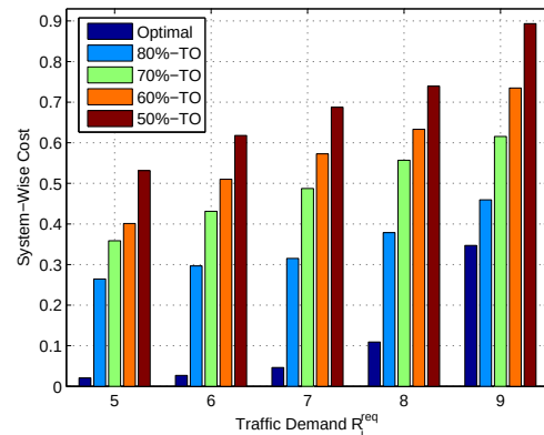
Fig. 9: Performance comparison with the fixed traffic scheduling scheme.
