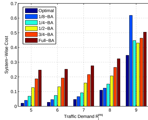
Fig. 8: Performance comparison with the fixed bandwidth scheme.
