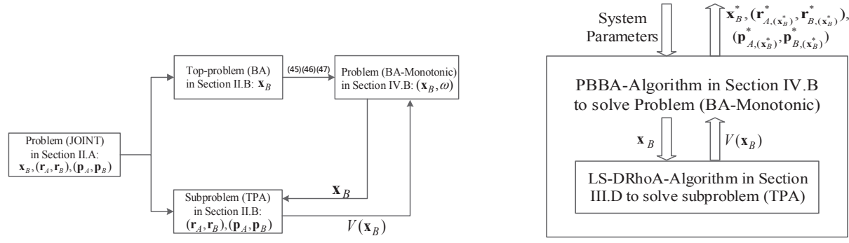
Fig. 3: Subfigure (a): Connections between top-problem (BA) and Problem (BA-Monotonic) regarding the decomposition of Problem (JOINT). Subfigure (b): Connections between our PBBA-Algorithm to solve Problem (BA-Monotonic) and the subroutine LS-DRhoA-Algorithm to solve subproblem (TPA).
