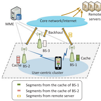
Fig. 1. Mobile edge caching with user-centric clustered services.
