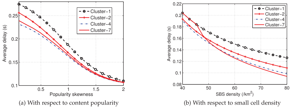
Fig. 8. Performance with different cluster size K .
