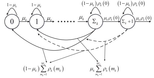
Fig. 2. Discrete-time Markov chain of the energy state at SBS.
