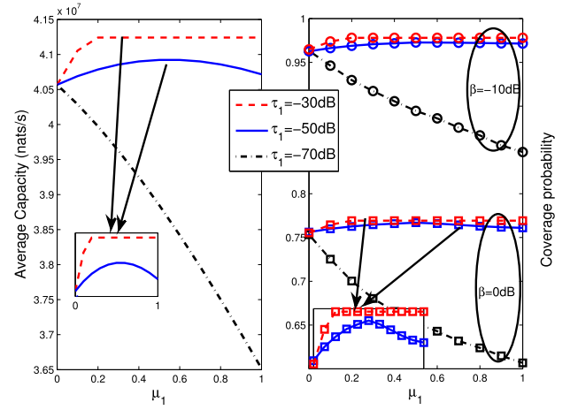
Fig. 7. Average capacity and coverage probability with respect to \mu .
