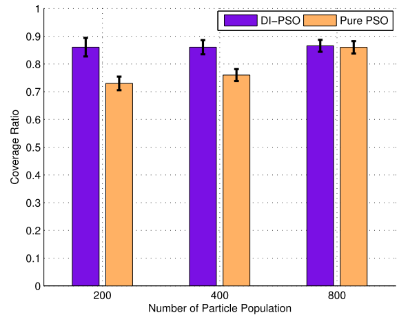
FIGURE 8. Performance comparison between pure PSO and DI-PSO algorithms with different particle populations.
