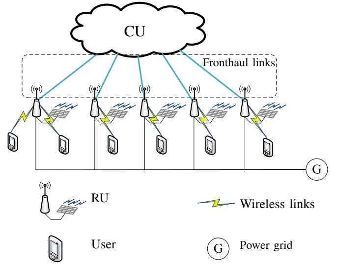
Fig. 1. HES-CRAN with energy harvesting and on-grid power supply.
