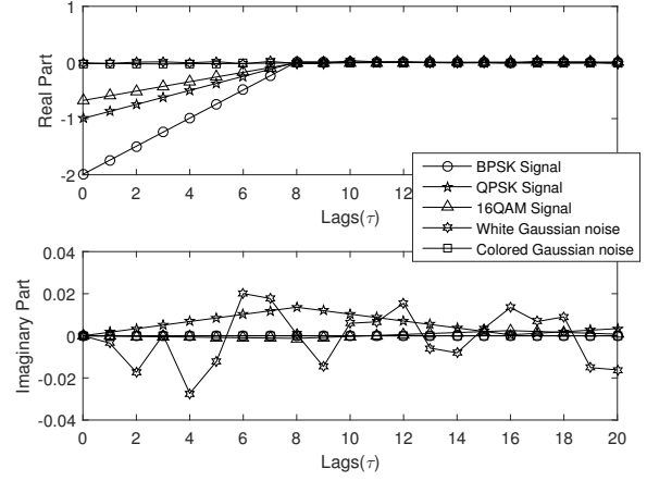
Fig. 3. Fourth-order cumulants of various random processes.
