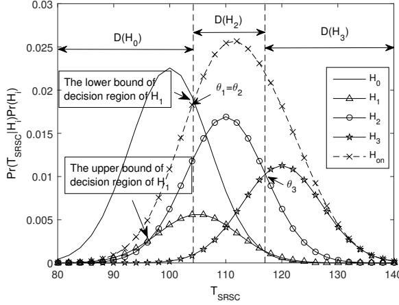
Fig. 2. Illustration for power mask effect in MPTP scenarios.
