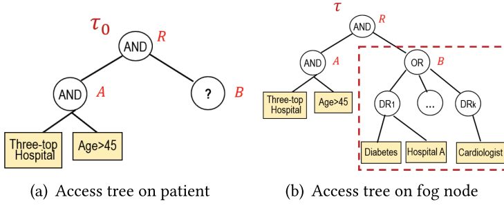
Fig. 3. Access tree construction.
