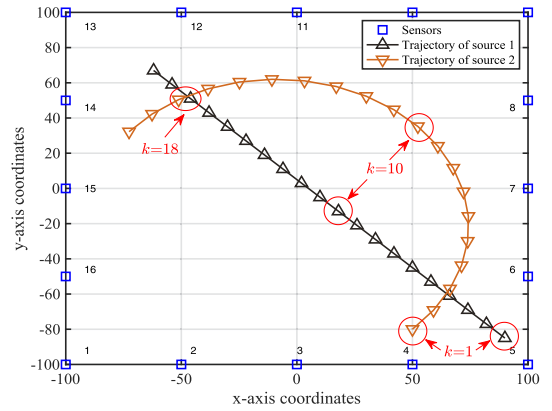
Fig. 10. Sensor network and trajectories of multiple sources.
