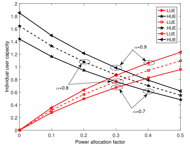
Fig. 5. User capacity based on BC-NOMA.
