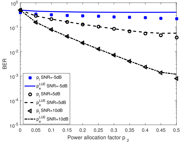
Fig. 6. p_\ell and p_e^{LUE} comparisons with different power allocation factor p_2 .
