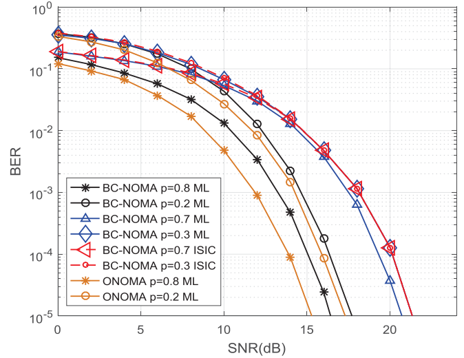
Fig. 10. BER performance in BC-NOMA and ONOMA system.
