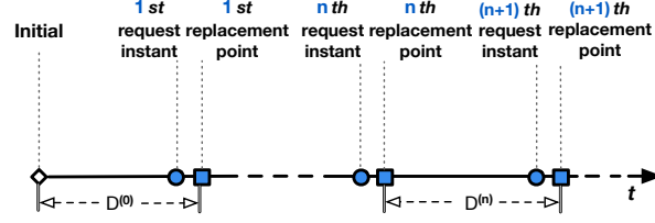
Fig. 1: Illustration of the timeline model. D^{(n)} represents the duration between the n th and the (n + 1) th replacement points.
