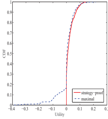
Fig. 13. CDF of vehicle utility.
