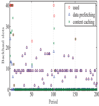
Fig. 7. Backhaul link utilization in each period.
