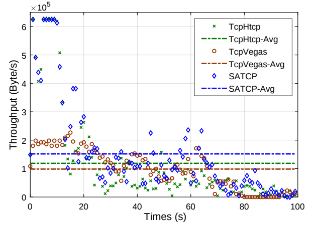
Fig. 5. Throughput comparisons
