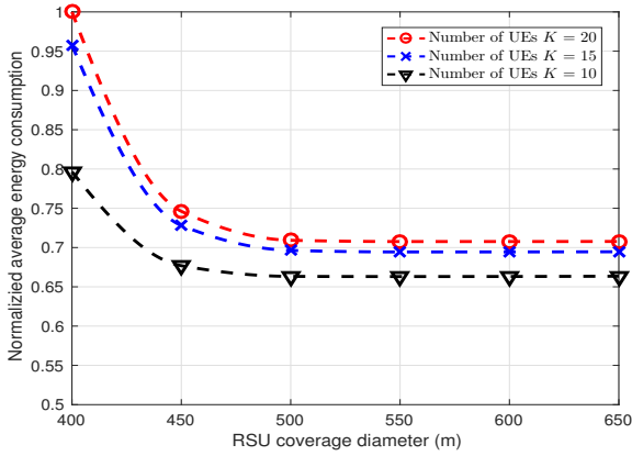
Fig. 6. Average energy consumption per UE versus RSU coverage diameter with different numbers of UEs. ( \bar{v}_k = 80\text{km/h} )
