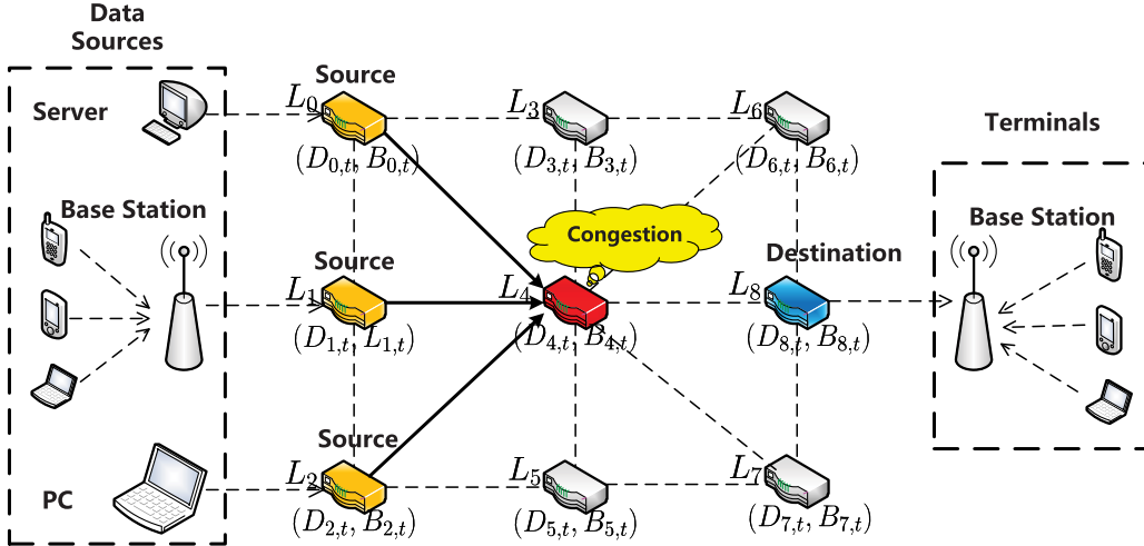
FIGURE 1. The network topology.
