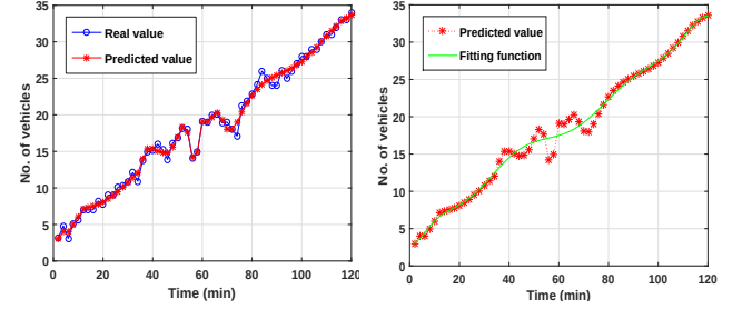
(a) ANN prediction with 20 epochs. (b) Least square fitting.
