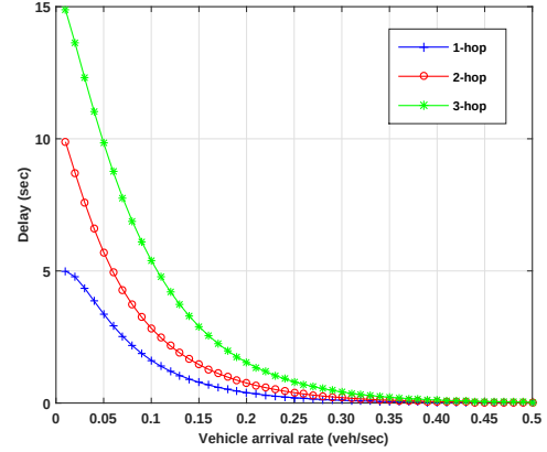
Fig. 8. V2V average delay.
