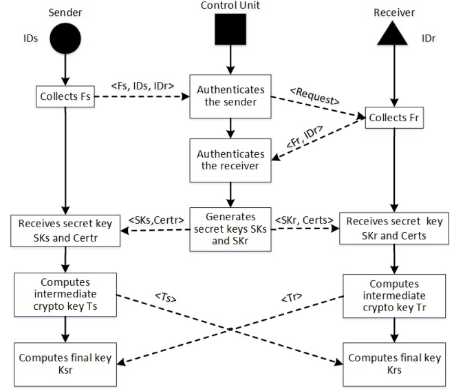
Fig. 1: Authenticated Key Agreement Process
