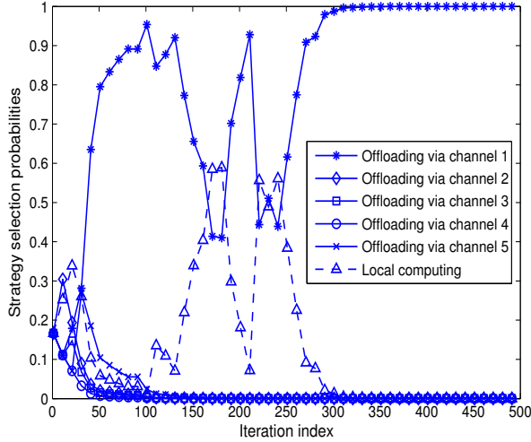
Fig. 3. Convergence of strategy selection probabilities.
