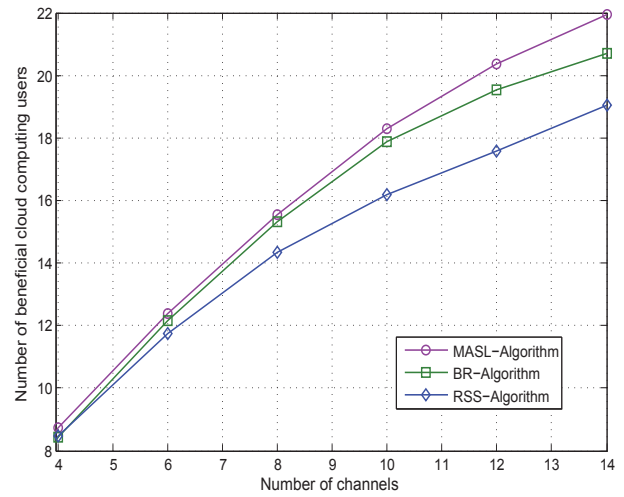
Fig. 10. Performance comparison in terms of beneficial cloud computing users for different numbers of channels.
