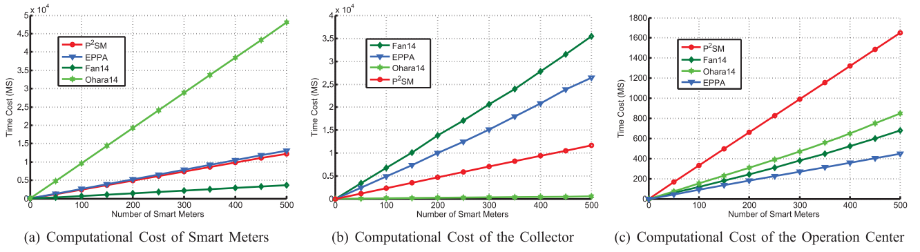
Fig. 3. Comparison on Computational Overhead.
