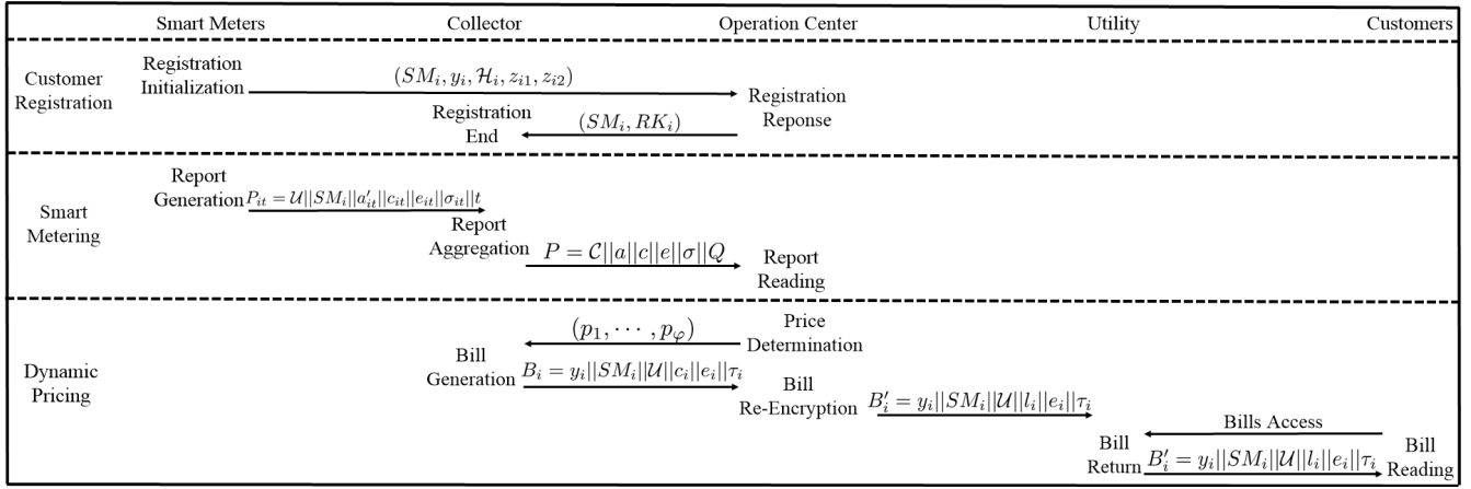
Fig. 2. Information Flow of P 2 SM.
