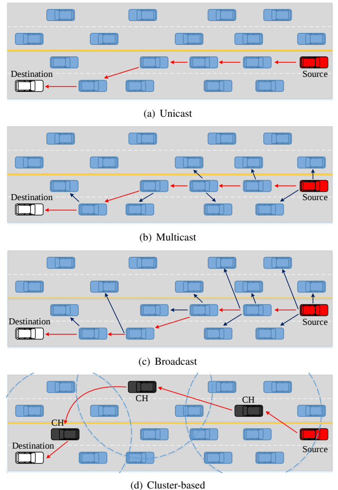
Figure 3. Illustration of four categories of routing protocol in MDVNETs.
