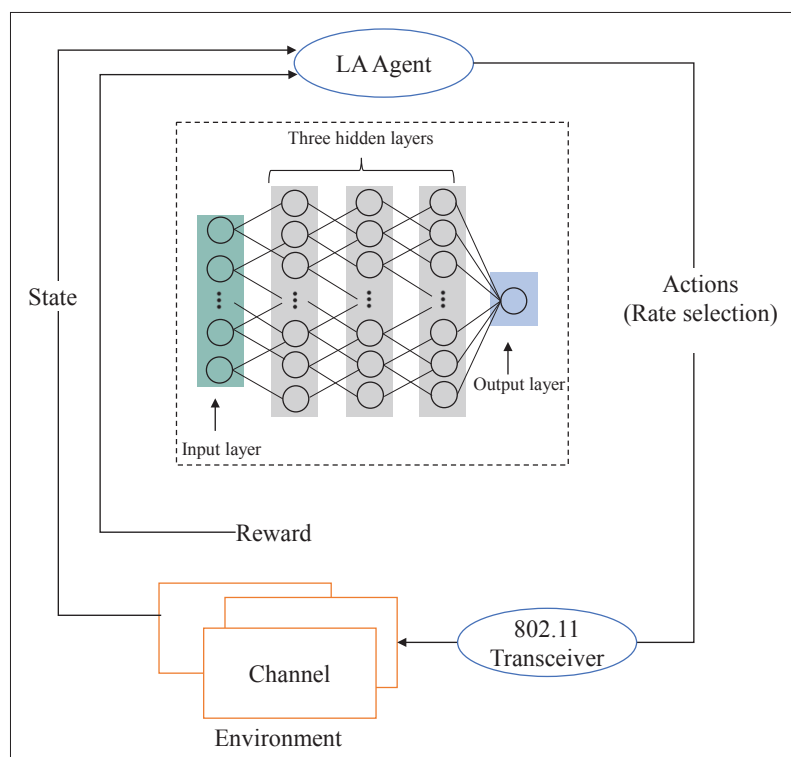
FIGURE 3. Deep learning model for LA in drive-thru Internet.
