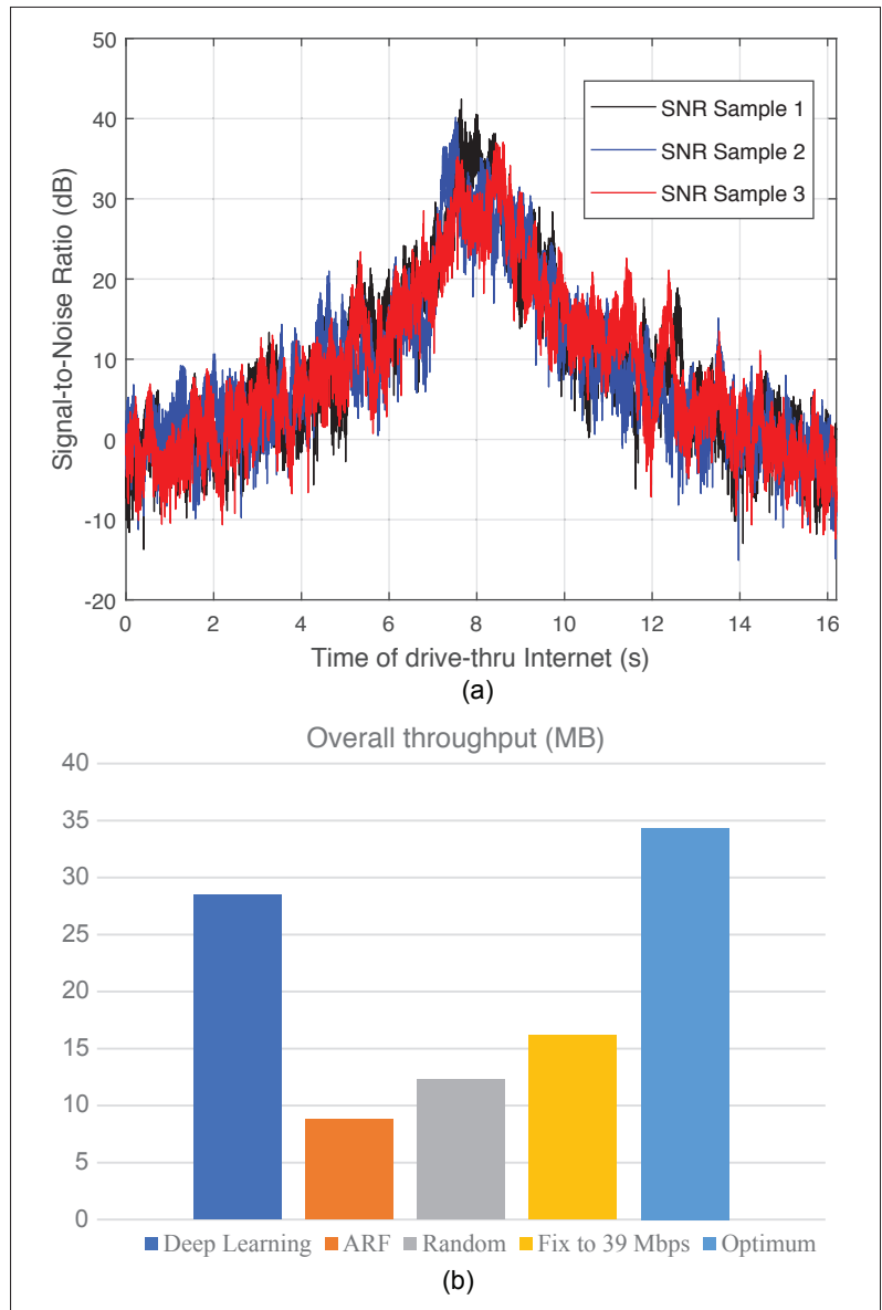
FIGURE 4. Data-driven learning-based LA in drive-thru Internet: a) drive-thru Internet channel snapshot; b) deep learning model-based LA performance.
