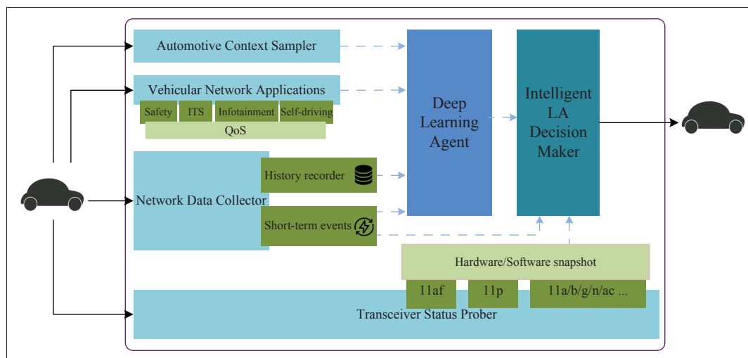
FIGURE 2. Data-driven intelligent LA architecture in 802.11 V2X.
