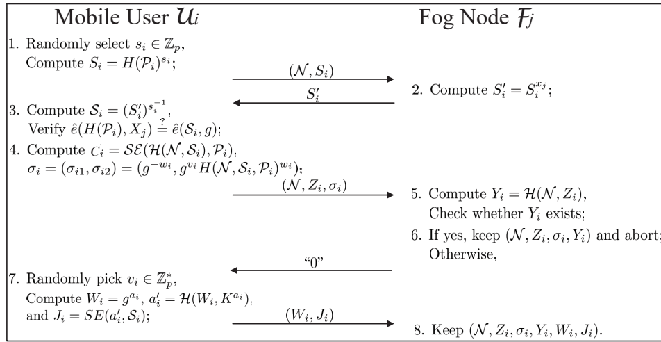
Fig. 3. Information Flow of Data Collection
