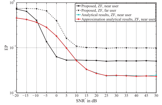
Fig. 3. PEP performance approximation of the ZF-ZF detector.
