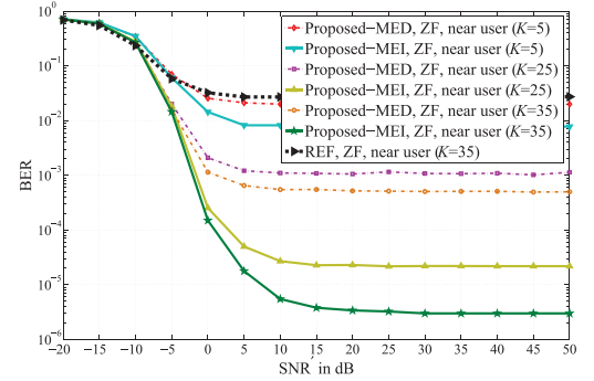
Fig. 9. BER versus \text{SNR}' for u_k where N = 4 and the ZF-ZF detector is employed.
