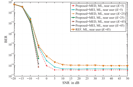
Fig. 7. BER versus \text{SNR}' for u_k where N = 4 and the ML-ML detector is employed.
