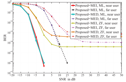
Fig. 4. BER versus SNR' with K = 5 , P = 5 , and M = N = 2 .
