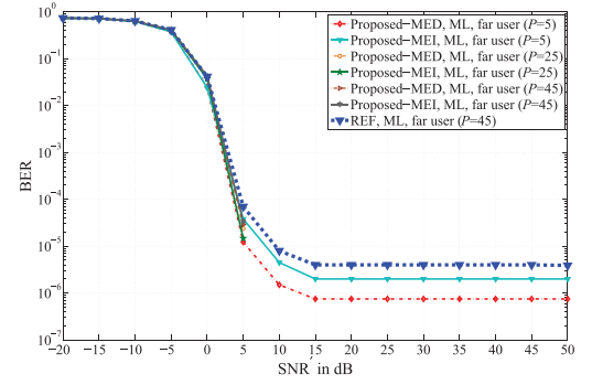
Fig. 8. BER versus \text{SNR}' for u_p where N = 4 and the ML-ML detector is employed.
