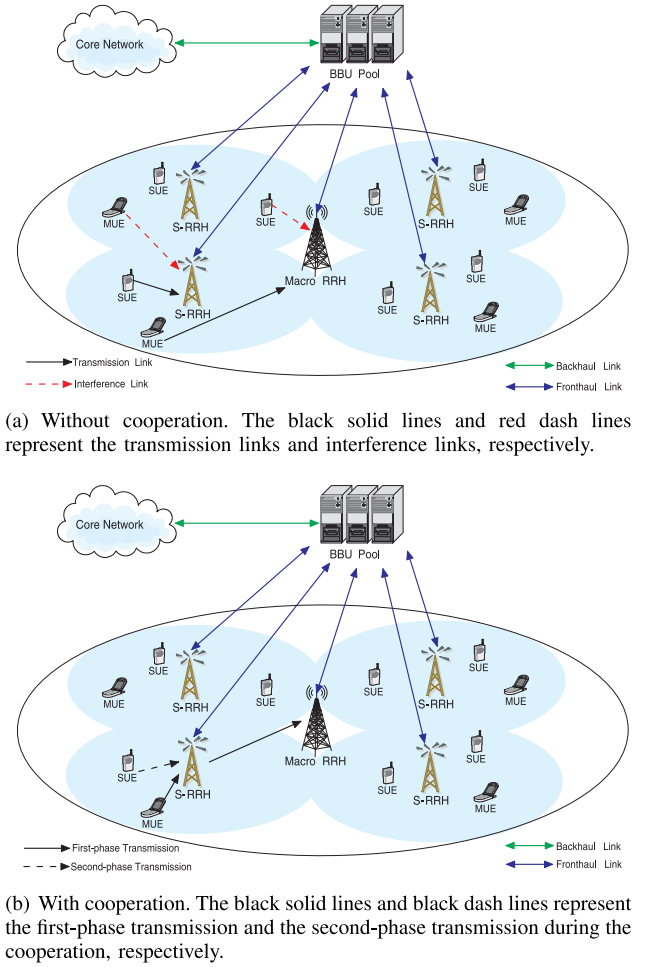
Fig. 1. The H-CRAN framework. The green link is the backhaul link between core network and BBU pool, and the blue links are the fronthaul links between BBU pool and RRHs.
