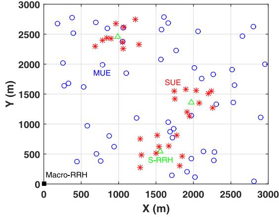
Fig. 3. H-CRAN deployment.
