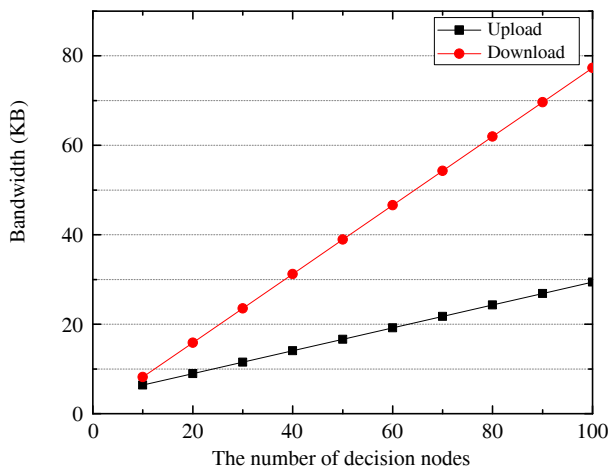
Figure 5 Bandwidth vs. the number of decision nodes
