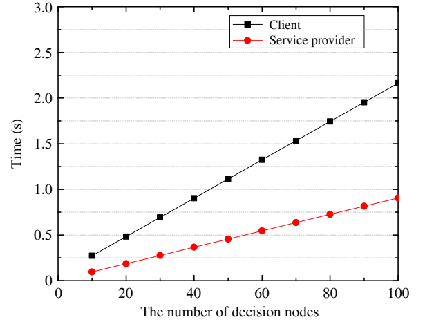
Figure 4 Computation cost vs. the number of decision nodes
