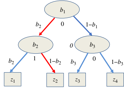
Figure 3 Edge cost of a decision tree
