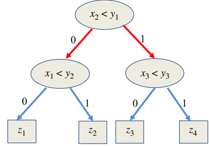
Figure 2 A decision tree
