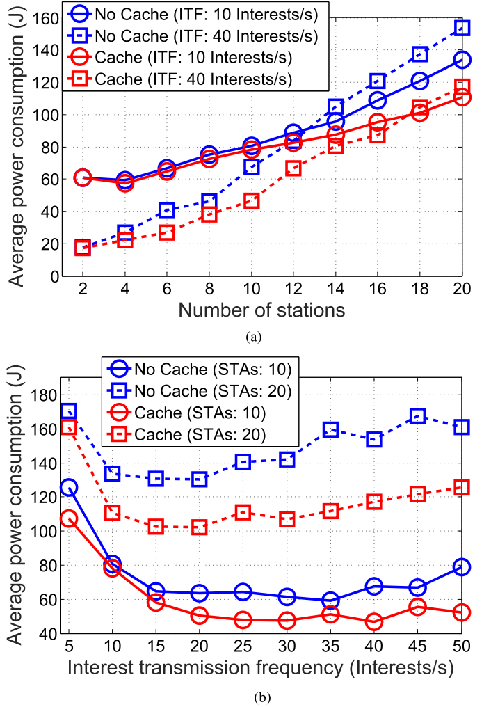
Fig. 13. Caching-aided NDN-PSM performance. (a) Power consumption vs. stations. (b) Power consumption vs. ITF.
