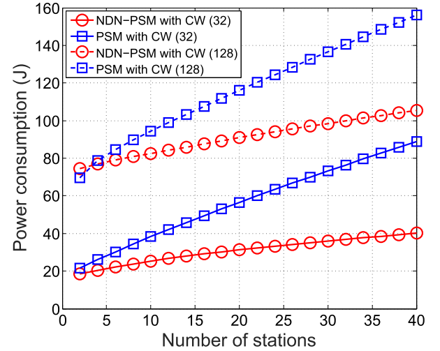
Fig. 8. Numerical results of power consumption.
