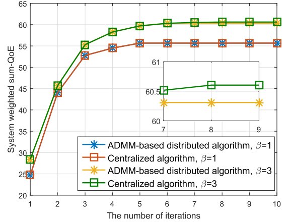
Fig. 5. Convergence behaviour of our proposed caching algorithms with P_m = 40 dBm.
