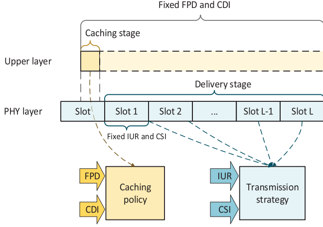
Fig. 2. The main structure of our proposed caching policy and transmission strategy. The caching policy is updated in the upper layer based on the statistical information and the transmission strategy is updated in the PHY layer based on the instantaneous information.
