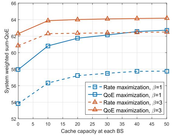
Fig. 12. The impact of transmission strategies (QoE maximization and Rate maximization) on the system weighted QoE with P_m = 40 dBm.
