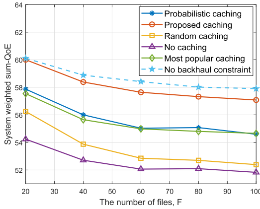
Fig. 10. The impact of cache placement on the system weighted sum-QoE with different number of video contents.
