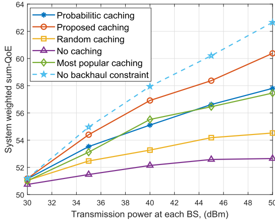
Fig. 7. The effect of cache placement on the system weighted sum-QoE with different transmission powers and S_m = 10 .
