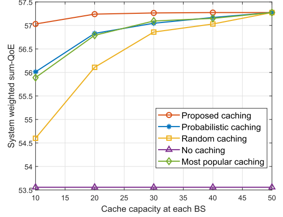
Fig. 8. The impact of cache placement on the system weighted QoE performance with different cache capacities and P_m = 40 dBm.
