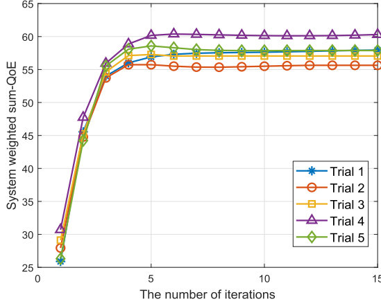
Fig. 6. Convergence behaviour of our proposed transmission algorithms with P_m = 40 dBm.
