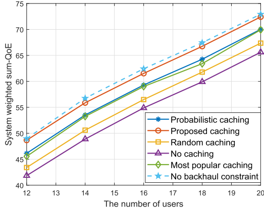
Fig. 9. The impact of cache placement on the system weighted sum-QoE with different number of users.
