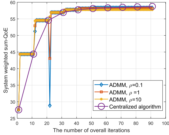
Fig. 4. Convergence behaviour of our proposed ADMM-based distributed cache placement algorithm with different \rho .
