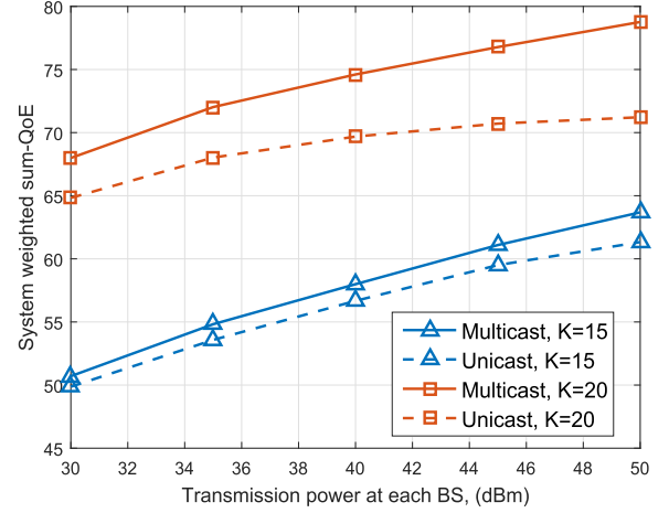
Fig. 11. The impact of transmission strategies (multicast and unicast) on the system weighted QoE with S_m = 10 .
