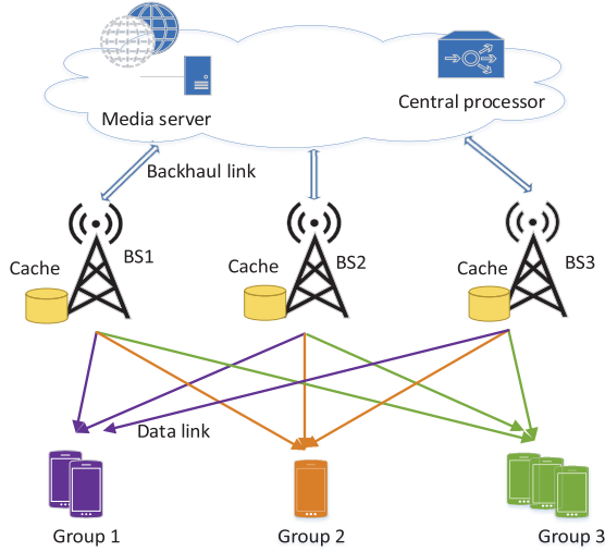
Fig. 1. An example of multicast transmission in a cache-enabled cloud-RAN. All users are formed as three multicast groups, which are cooperatively served by all BSs.
