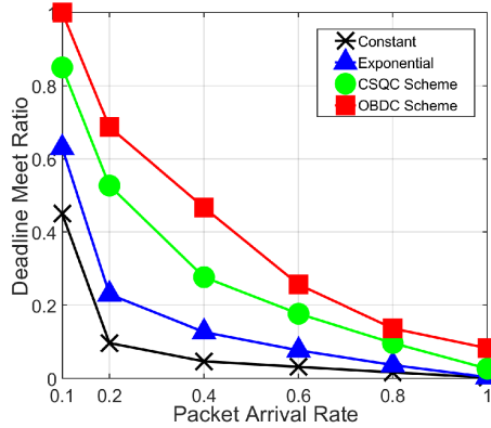
Fig. 14. DMR vs. packet arrival rate.
