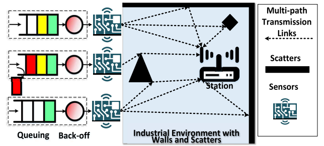
Fig. 1. Network model.
