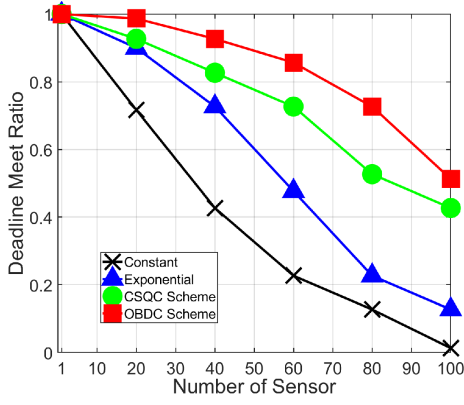
Fig. 12. DMR vs. number of sensor.
