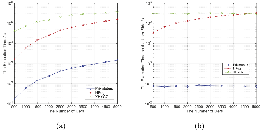
Fig. 6. (a) The execution time of schemes; (b) The execution time of schemes on the user side, on the smartphones and the server.
