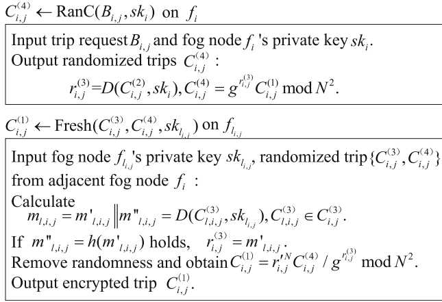
Fig. 5. Fog node-to-fog node interaction.
