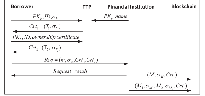
Fig. 3. Interaction process of BAPIM.
