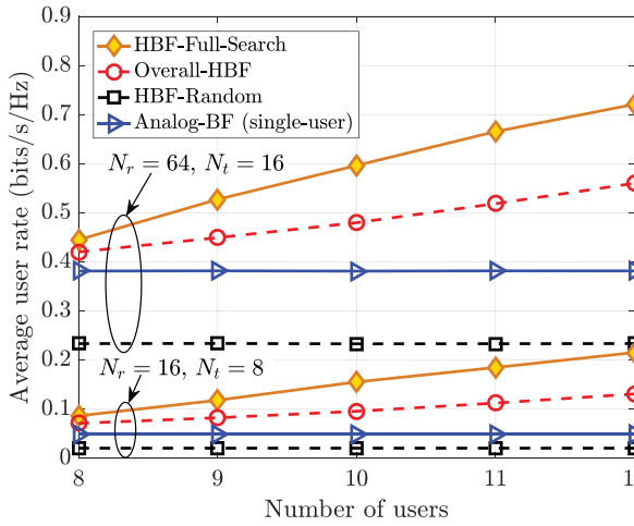
Fig. 10. Average user rate versus the number of users ( n = 2.17 , \text{SNR} = 30 dB, S \leq 4 , N_f = S ).
