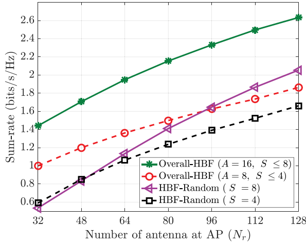
Fig. 13. Sum rate versus the number of AP[’s] antennas ( K = 32 , N_t = 16 , n = 2.17 SNR = 30 dB, N_f = S ).
