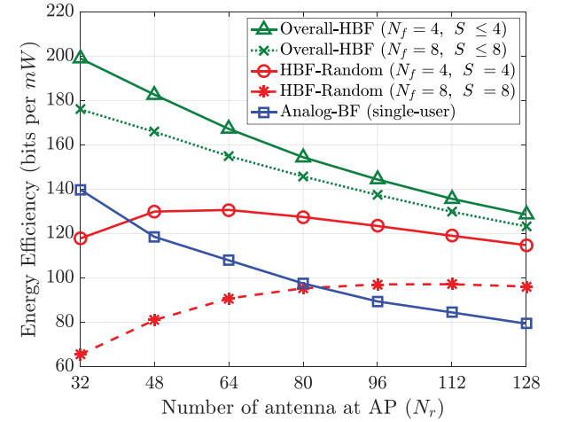
Fig. 15. Energy efficiency performance at the AP versus the number of antennas ( K = 32 , N_t = 16 , n = 2.17 SNR = 30 dB).
