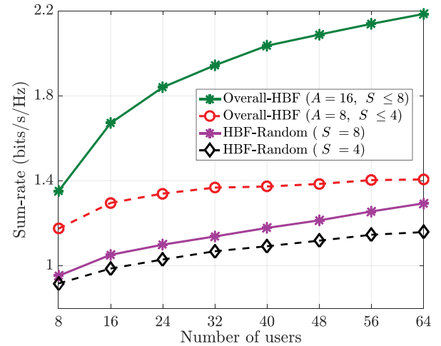
Fig. 12. Sum rate versus the number of users ( N_r = 64 , N_t = 16 , n = 2.17 , \text{SNR} = 30 dB, N_f = S ).
