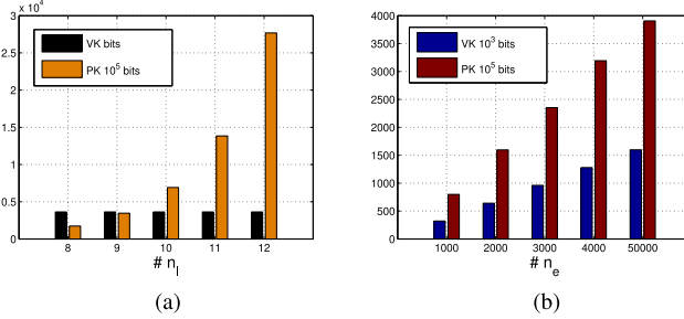
Fig. 6. CRS Size. (a) \mathcal{F}_R . (b) \mathcal{F}_T .
