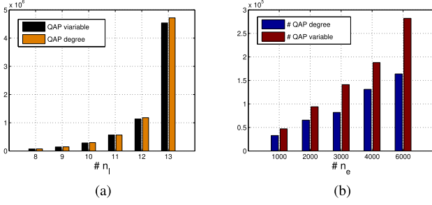
Fig. 5. QAP Complexity. (a) \mathcal{F}_R . (b) \mathcal{F}_T .
