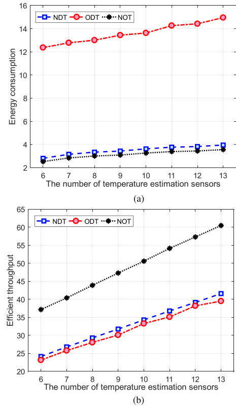
Fig. 7. Transmission performance comparison among different numbers of temperature-estimation sensors. (a) Energy consumption. (b) Efficient throughput.
