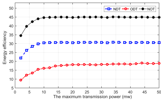
Fig. 6. The energy efficiency with different maximum transmission power.
