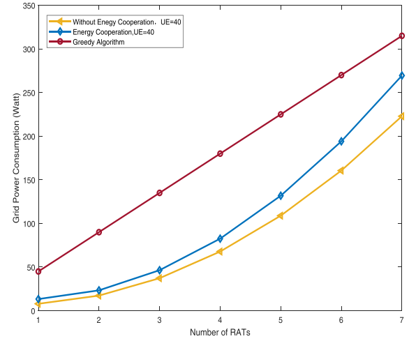
Fig. 6. Grid power consumption V.S. number of RATs.
