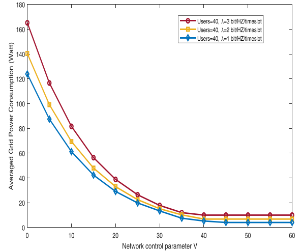
Fig. 4. Grid power consumption with parameter V .
