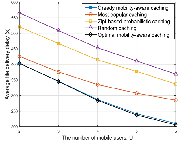
Fig. 3. Average file delivery delay versus the number of mobile users with F = 20 , C = 0.2 GB, \beta = 0.6 , N = 5 and N_c = 2 .
