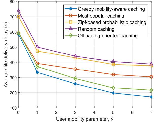
Fig. 9. Average file delivery delay versus the user mobility parameter with F = 50 , U = 20 , C = 0.2 GB, \beta = 0.6 , N = 5 and N_c = 2 .
