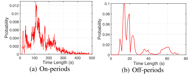
Fig. 4. Distributions of on-off periods for TVWS transmission.
