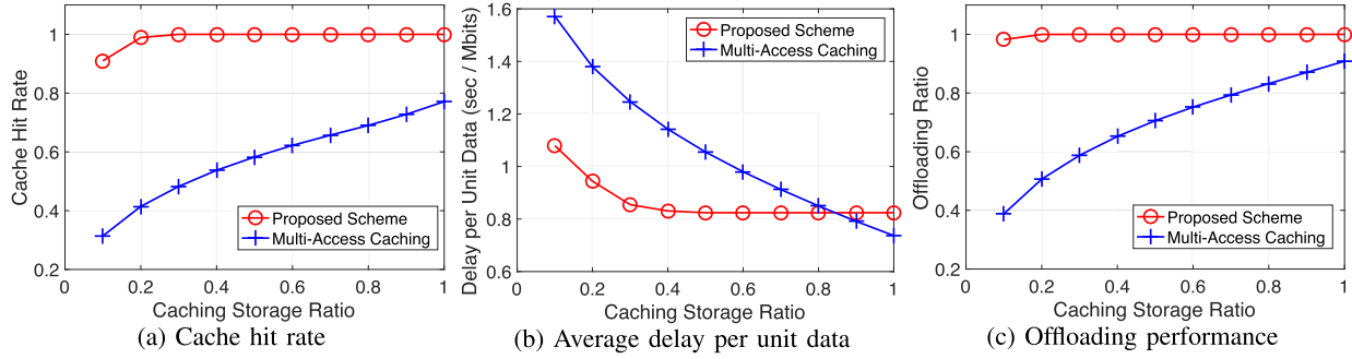
Fig. 8. Cache hit rate, delay, and offloading performance comparison between the proposed scheme and multi-access-based caching scheme.
